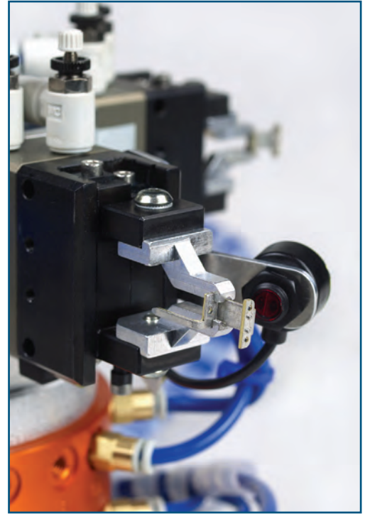
Miniature Part Placement Tool
