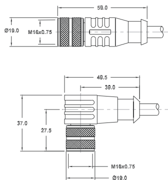
Female 14-Pin M16 x 0.75
