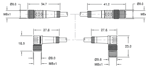
3-Pin Sensor Cables
