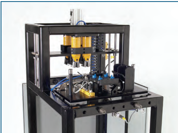
Punch Press Degater w/ Interchangeable Part Nests and Heated Cutting Steel.
