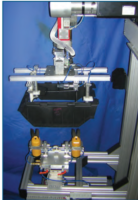
Rotary Degate Station reduces number of cutters and blades needed.
