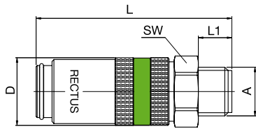
Male Thread
