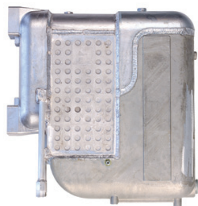
Polestar Smartpack, all-in-one aluminium heat-exchanger
