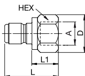
Female Thread
